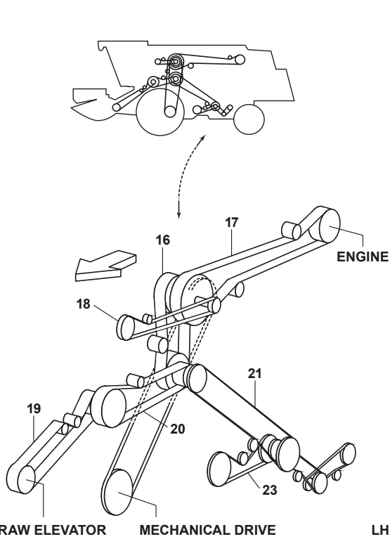
STRAW ELEVATOR MECHANICAL DRIVE LH
