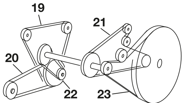
TX 66 (RH)
