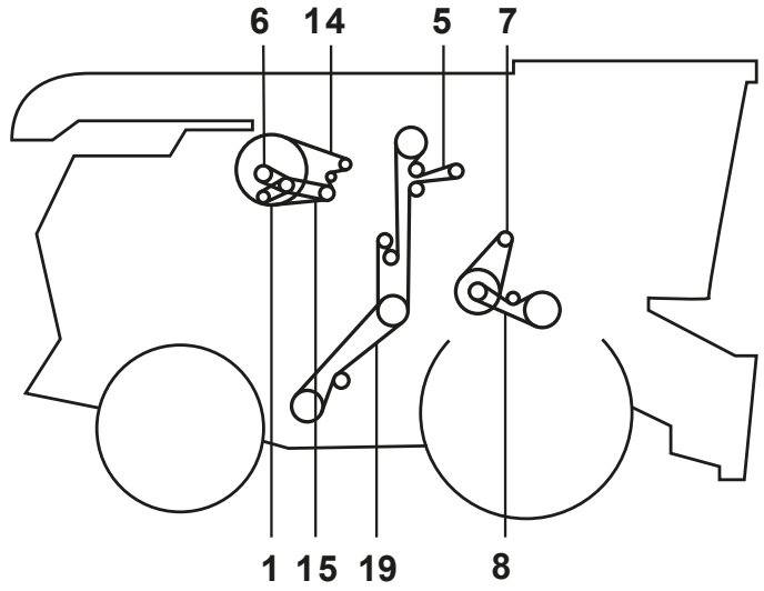
Feederhouse Fixed W/Reverser
