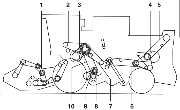
CUTTER PKN1500B
