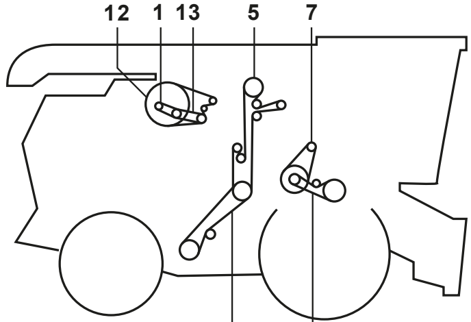
Feederhouse Fixed W/Reverser
