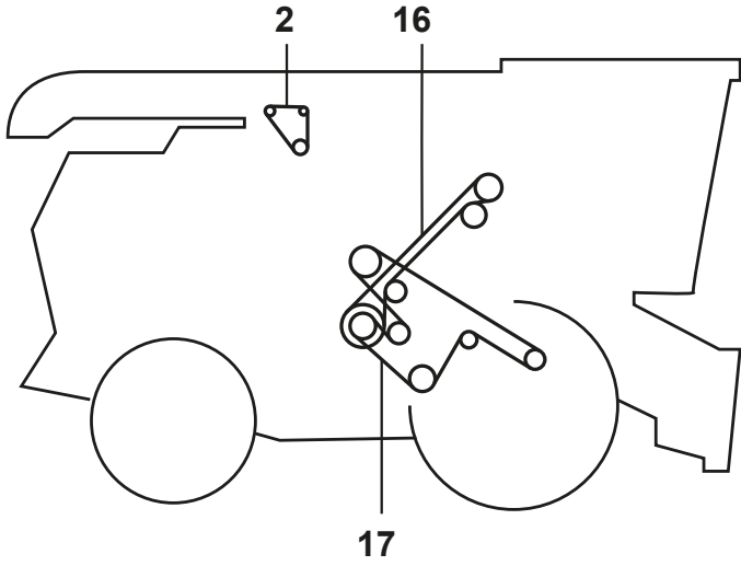
Straw Spreader
