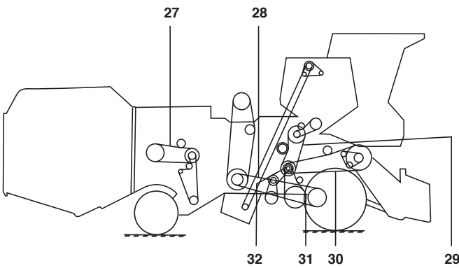
WITH MECHANICAL DRIVE UNDERCARRIAGE AND STACKER
